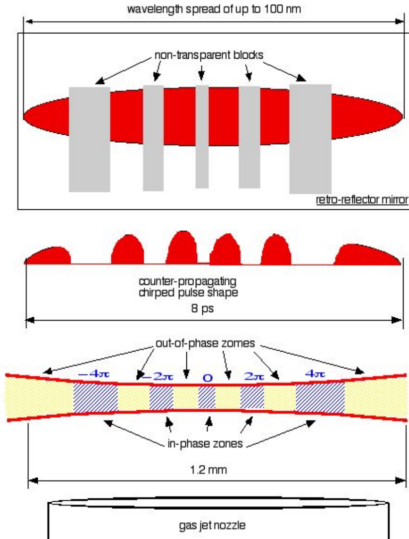
Fig. 5.5 Elimination of harmonic production (harmonic order in the upper thirties) in the “out-of-phase” regions using a train of counter-propagating pulses created by removing spectral regions of a chirped pulse.
