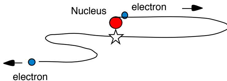
Fig. 1.6 Return of an electron to the atomic center, positioned at x=0 .
